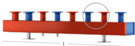
Compact manifold, thermally separated
